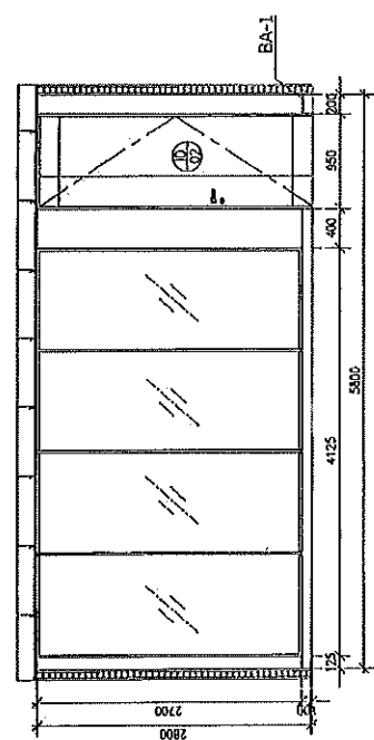
ELEVATION 1 SCALE 1 : 50
