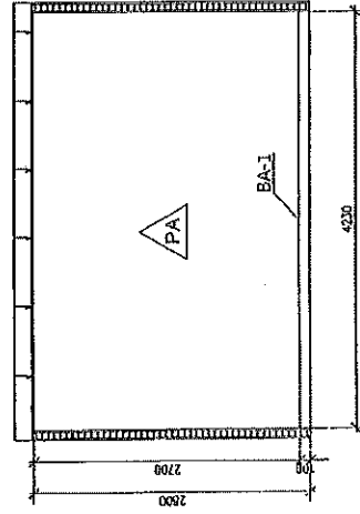
ELEVATION 1 SCALE 1 : 50
