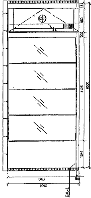
ELEVATION 3 SCALE 1 : 50
