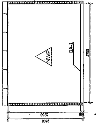
ELEVATION 2 SCALE 1 : 50
