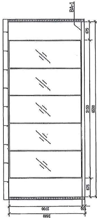
ELEVATION 1 SCALE 1 : 50
