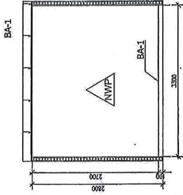
ELEVATION 4 SCALE 1 : 50
