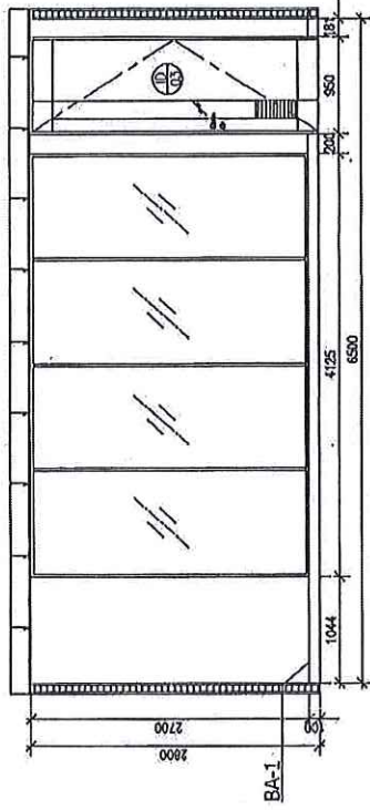
ELEVATION 3 SCALE 1 : 50
