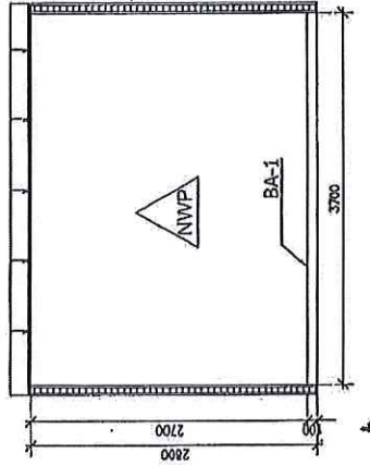
ELEVATION 2 SCALE 1 : 50
