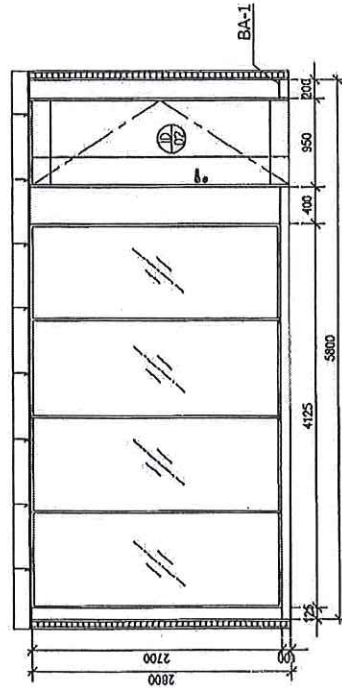
ELEVATION 1 SCALE 1 : 50
